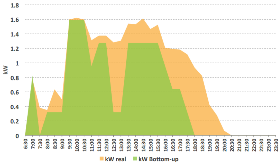
Figure 16: Lighting appliances load example in class amphitheatre
