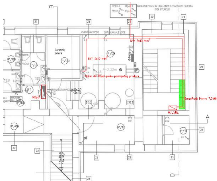
Figure 5: Battery system position
