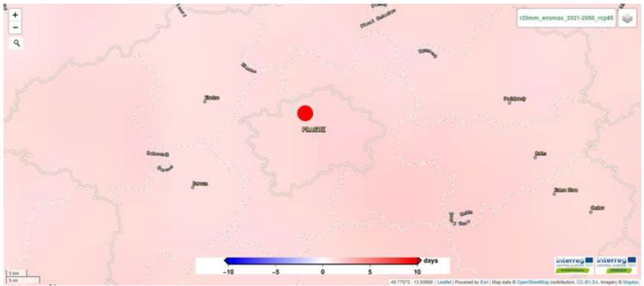
Near future (2021-2050) climate projections for Troja hamlet: R20mm RCP4.5 (above) and RCP8.5 (below).
