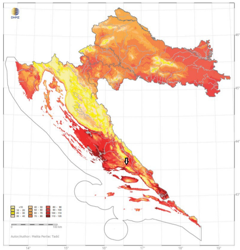
Mean annual number of warm days ( t_{max} \geq 25^{\circ}\text{C} )
