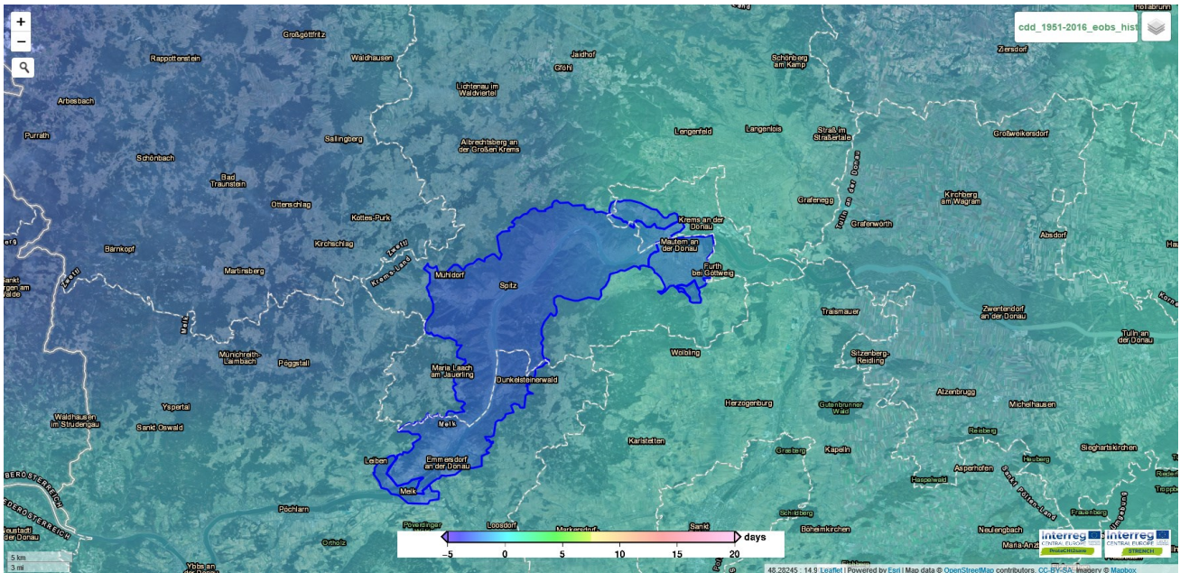
Figure 29 Historical Observation 1951 – 2016, WebGIS tool. (CCD)
