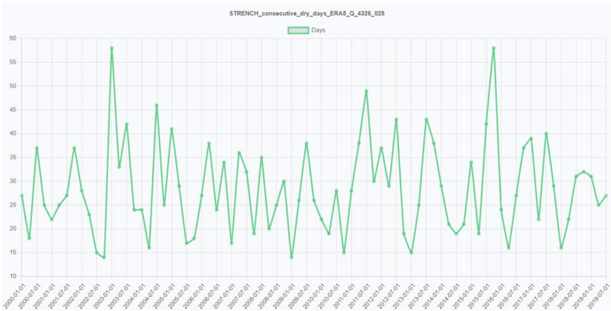
Consecutive dry days (ERA5) in the period of 2000-2019
