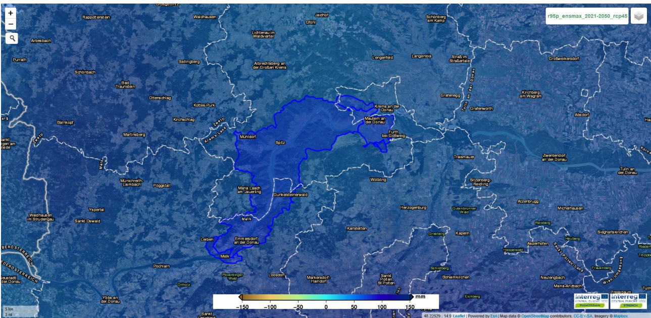
Figure 24 Ensemble statistics, maximum, RCP 4.5 Near Future (2021 – 2050), WebGIS tool. (R95pTOT)
