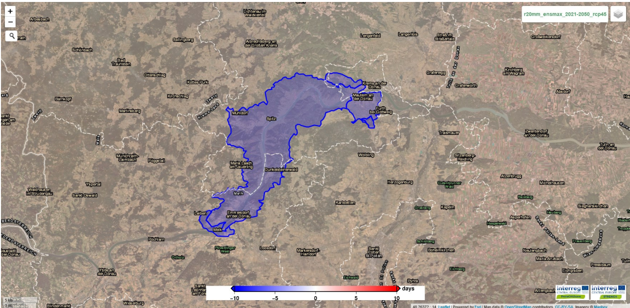
Figure 21 Ensemble statistics, maximum, RCP 4.5 Near Future (2021 – 2050), WebGIS tool. (R20mm)
