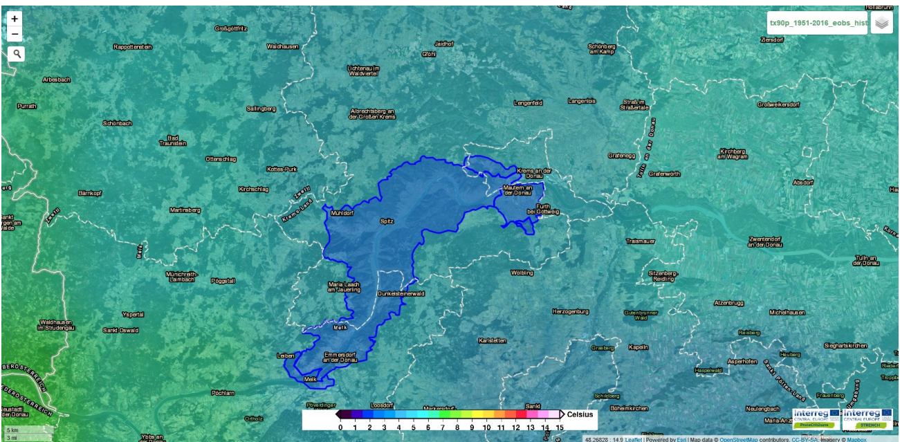
Figure 32 Historical Observation 1951 – 2016 in Celsius, WebGIS tool. (Tx90p)
