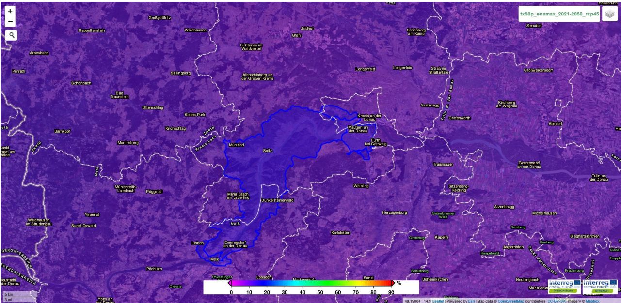
Figure 33 Ensemble statistics, maximum, RCP 4.5 Near Future (2021 – 2050). Not in Celsius but in percentage, WebGIS tool. (Tx90p)
