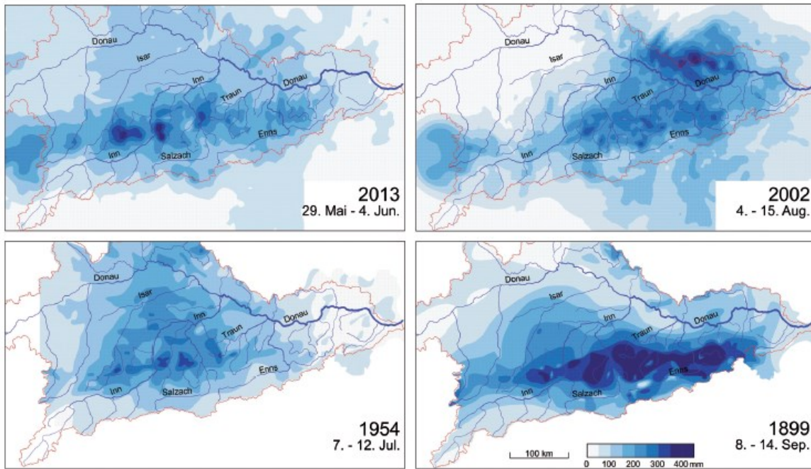
Figure 15 Event precipitation of the four floods in the Danube catchment in the past two centuries
