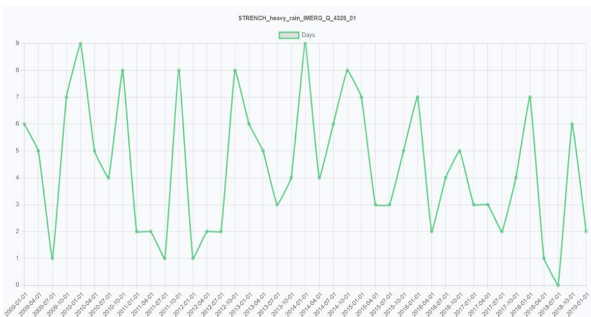
Heavy rain days (R20mm - IMERG) in the period of 2009-2019
