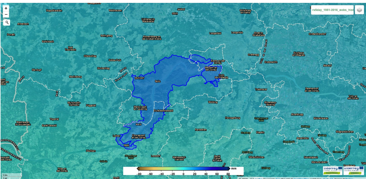
Figure 26 Historical Observation 1951 – 2016, WebGIS tool. (Rx5day)
