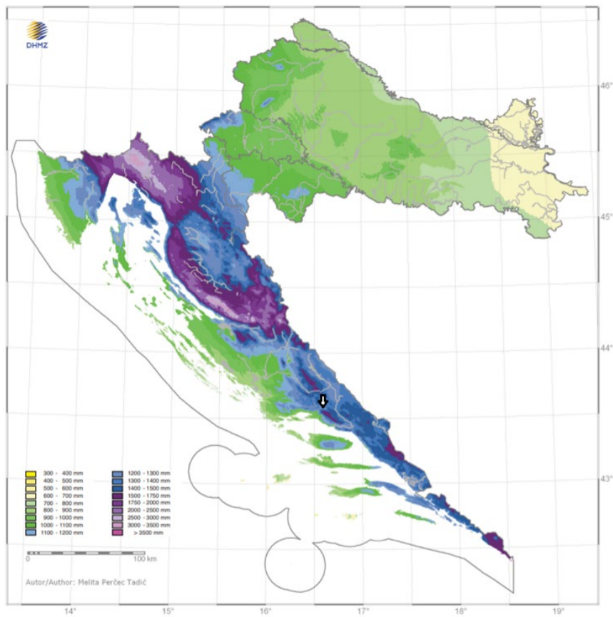
Mean annual precipitation
