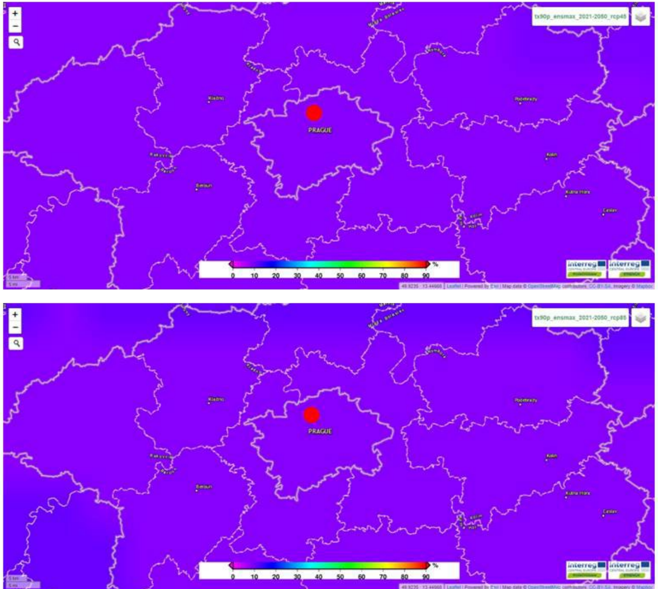
Near future (2021-2050) climate projections for Troja hamlet: Tx90p RCP4.5 (above) and RCP8.5 (below).
