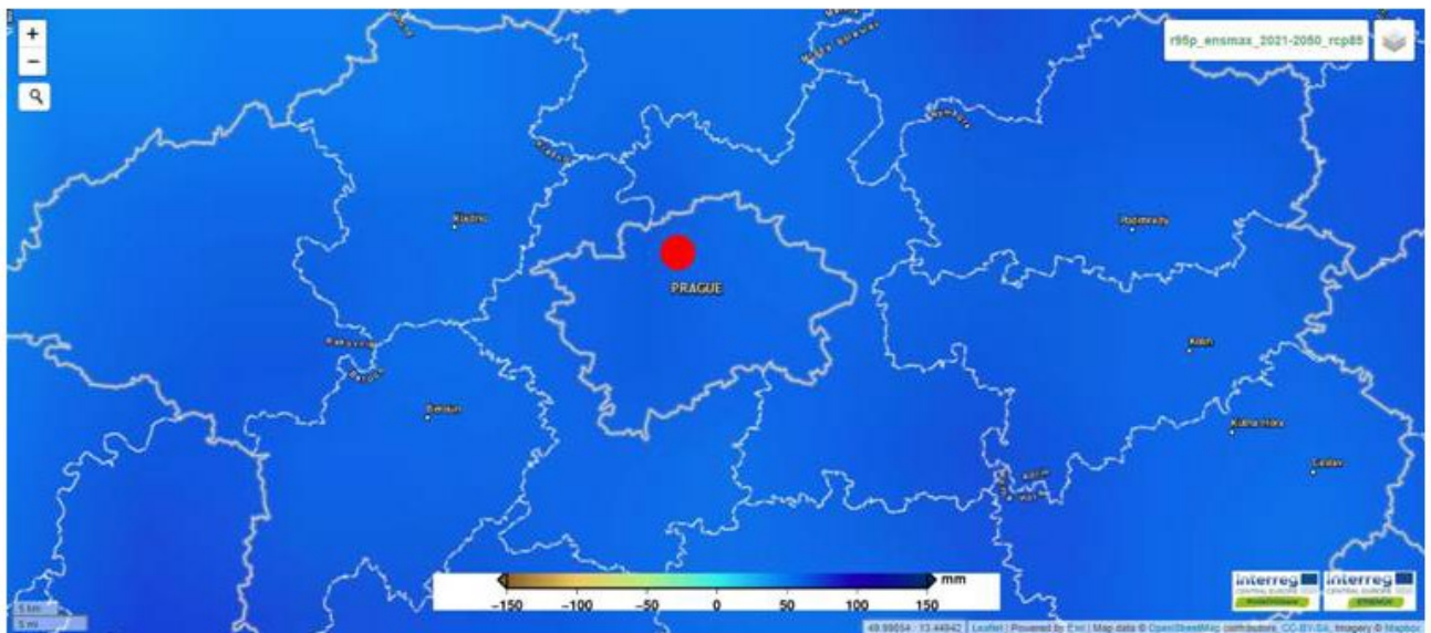
Near future (2021-2050) climate projections for Troja hamlet: R95p RCP4.5 (above) and RCP8.5 (below).
