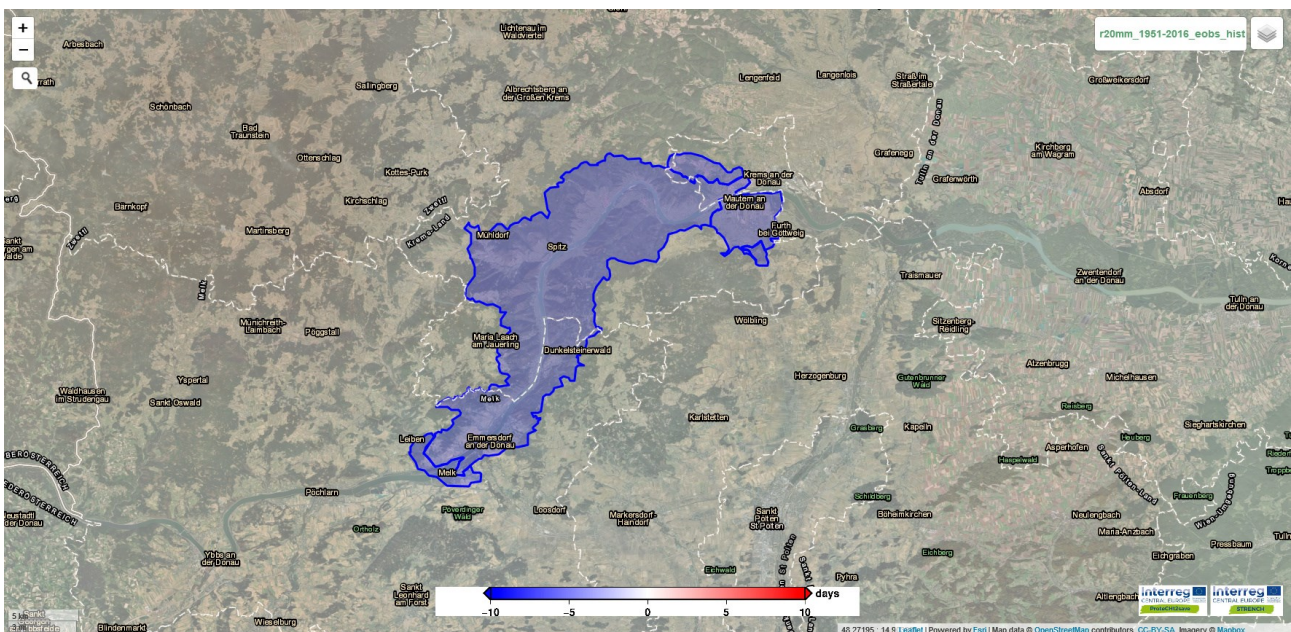
Figure 20 Historical Observation 1951 – 2016, WebGIS tool. (R20mm)
