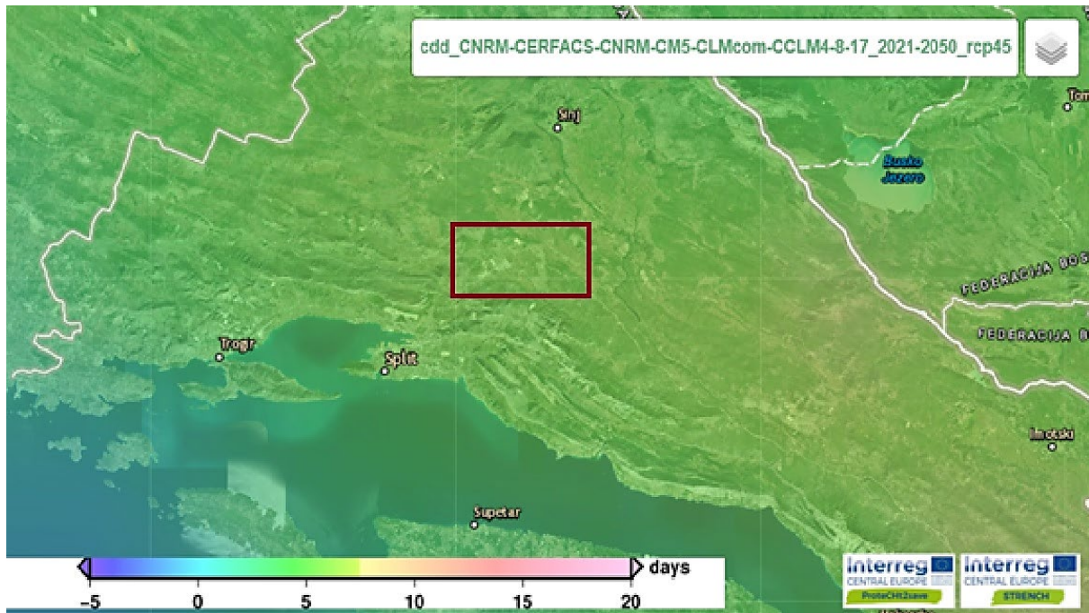
Near future (2021.-2050., RCP 4.5)
