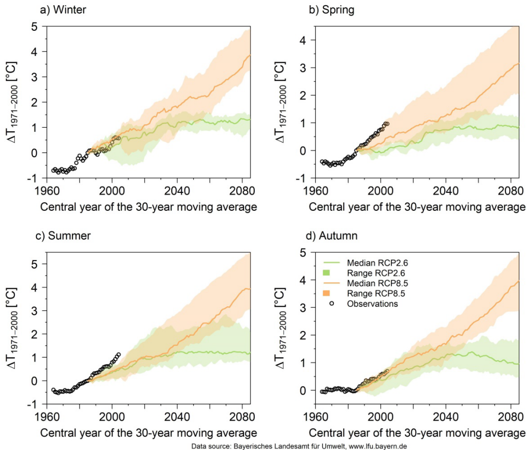
Figure 3: Climate projection of the 30-year moving average of the temperature anomaly (reference period: 1971-2000) for the climatic region of the DoF following RCP2.6 and RCP8.5 considering the seasons winter (Dec-Feb) a), spring (Mar-May) b), summer (Jun-Aug) c) and autumn (Sept-Nov) d).
