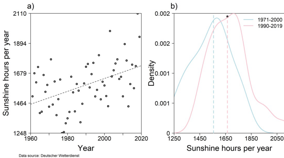
Figure 4: Temporal development of annual sunshine duration at a climate station in the DoF a), and frequency distribution of annual sunshine duration considering the climatic periods 1971-2000 and 1990-2019 b). The coloured dashed lines illustrate the median of the respective climatic period. The linear regression line and the * symbol were only displayed when statistical significance was observed.
