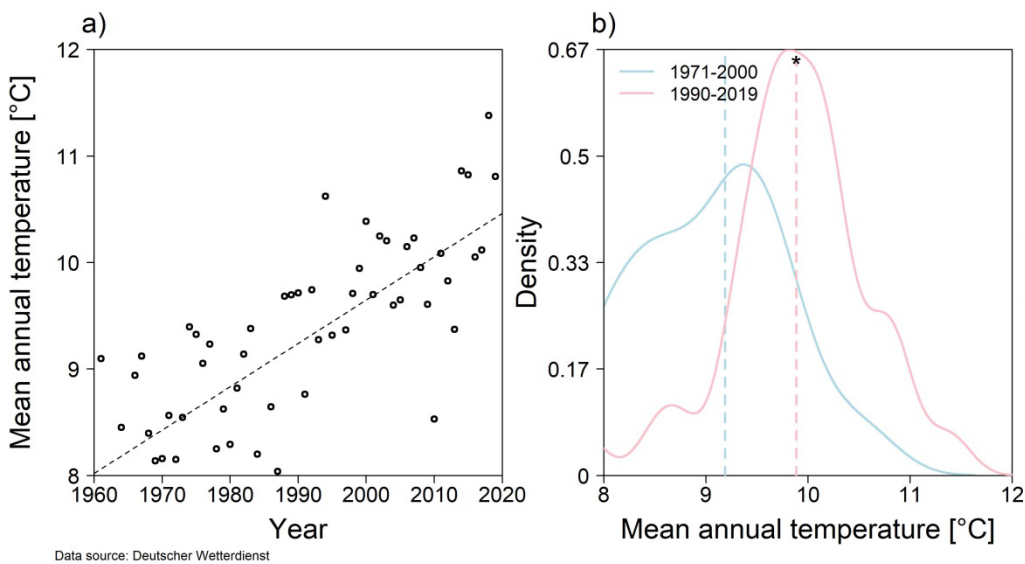
Figure 2: Temporal development mean median annual temperature at a climate station in the District of Forchheim a) and frequency distribution of mean median annual temperature considering the two climate periods 1971-2000 and 1990-2019 b). The coloured dashed lines illustrate the median of the respective climate period. The linear regression line and the * symbol were only displayed when statistical significance was observed.
