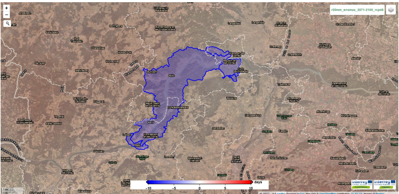
Figure 22 Ensemble statistics, maximum, RCP 4.5 Far Future (2071 – 2100), WebGIS tool. (R20mm)
