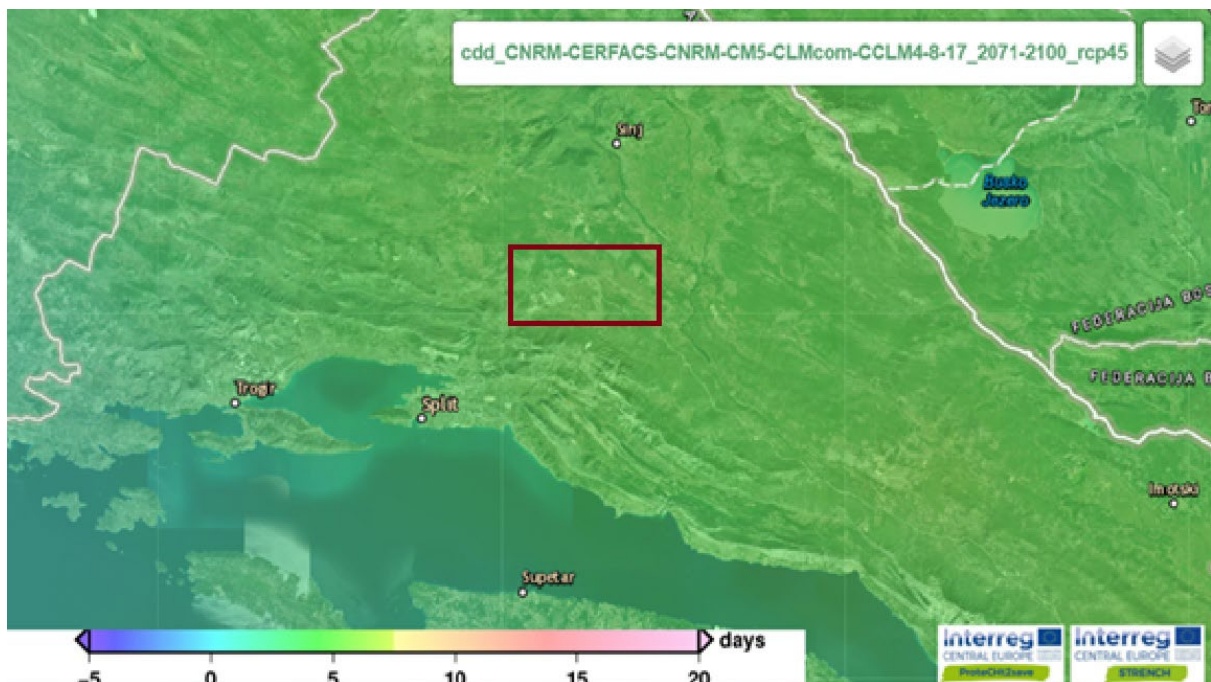
Far future (2071.-2100., RCP 4.5)
