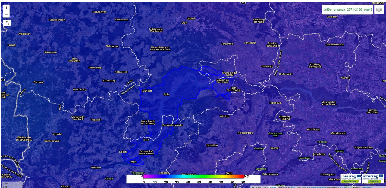
Figure 34 Ensemble statistics, maximum, RCP 4.5 Far Future (2071 – 2100). Not in Celsius but in percentage, WebGIS tool. (Tx90p)
