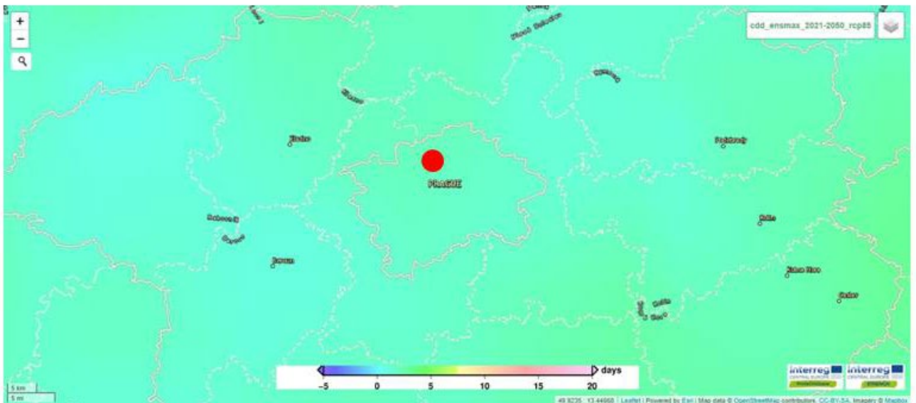
Near future (2021-2050) climate projections for Troja hamlet: CDD RCP4.5 (above) and RCP8.5 (below).
