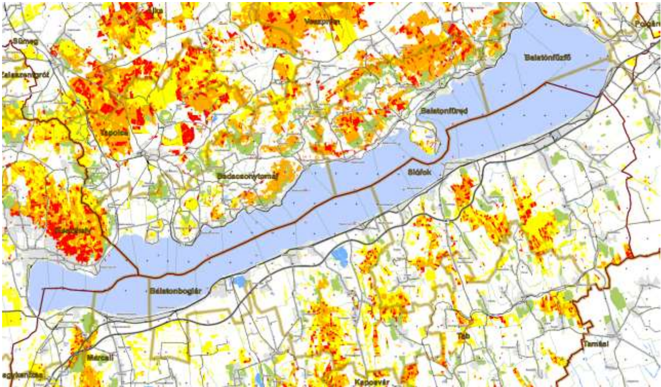
Fire risk map of the Lake Balaton area. Legend: red = forestal areas with high fire risk, orange = forestal areas with moderate fire risk, yellow = forestal areas with no fire risk.
