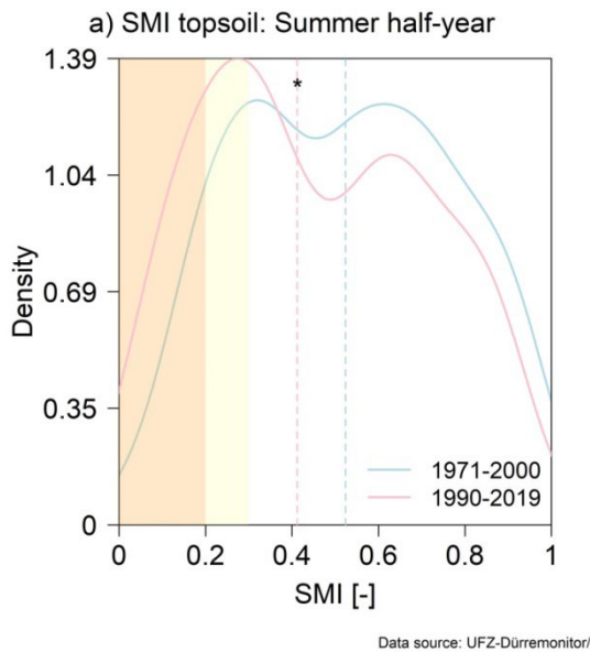
Figure 6: Frequency distributions of the top-soil SMI in the DoF considering the two climatic periods 1971-2000 and 1990-2019. The coloured dashed lines illustrate the median of the respective climatic period. The * symbol is only displayed when statistical significance was observed
