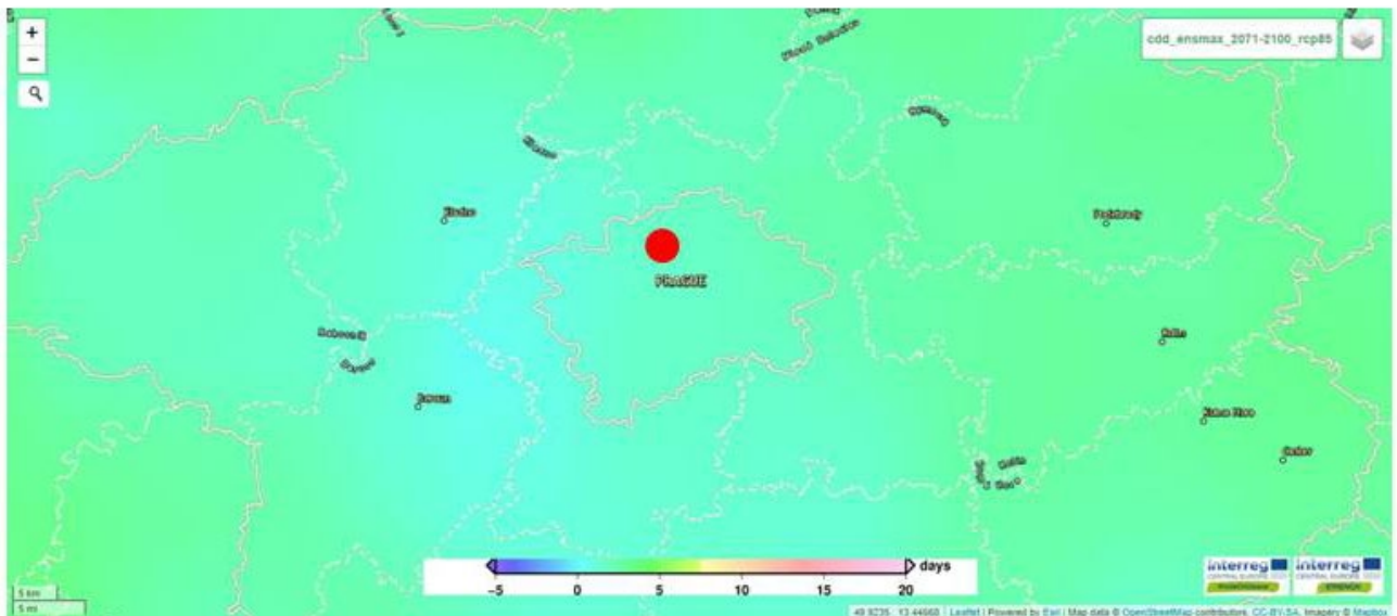
Far future (2071-2100) climate projections for Troja hamlet: CDD RCP4.5 (above) and RCP8.5 (below).
