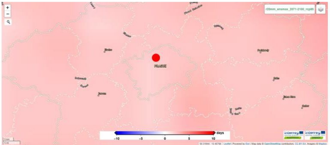
Far future (2071-2100) climate projections for Troja hamlet: R20mm RCP4.5 (above) and RCP8.5 (below).
