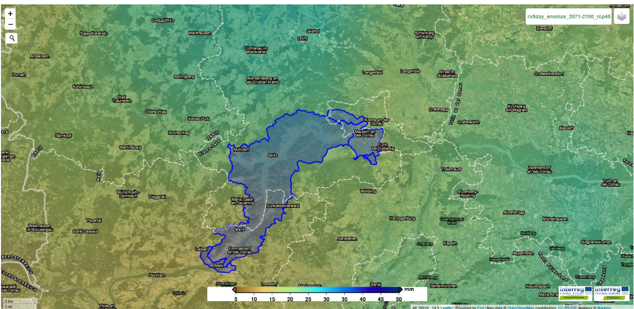
Figure 28 Ensemble statistics, maximum, RCP 4.5 Far Future (2071 – 2100), WebGIS tool. (Rx5day)
