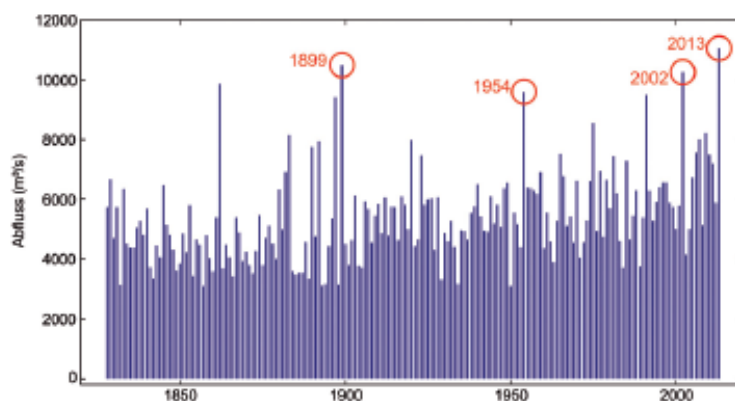
Figure 14 Annual floods of the Danube at Vienna since 1828
