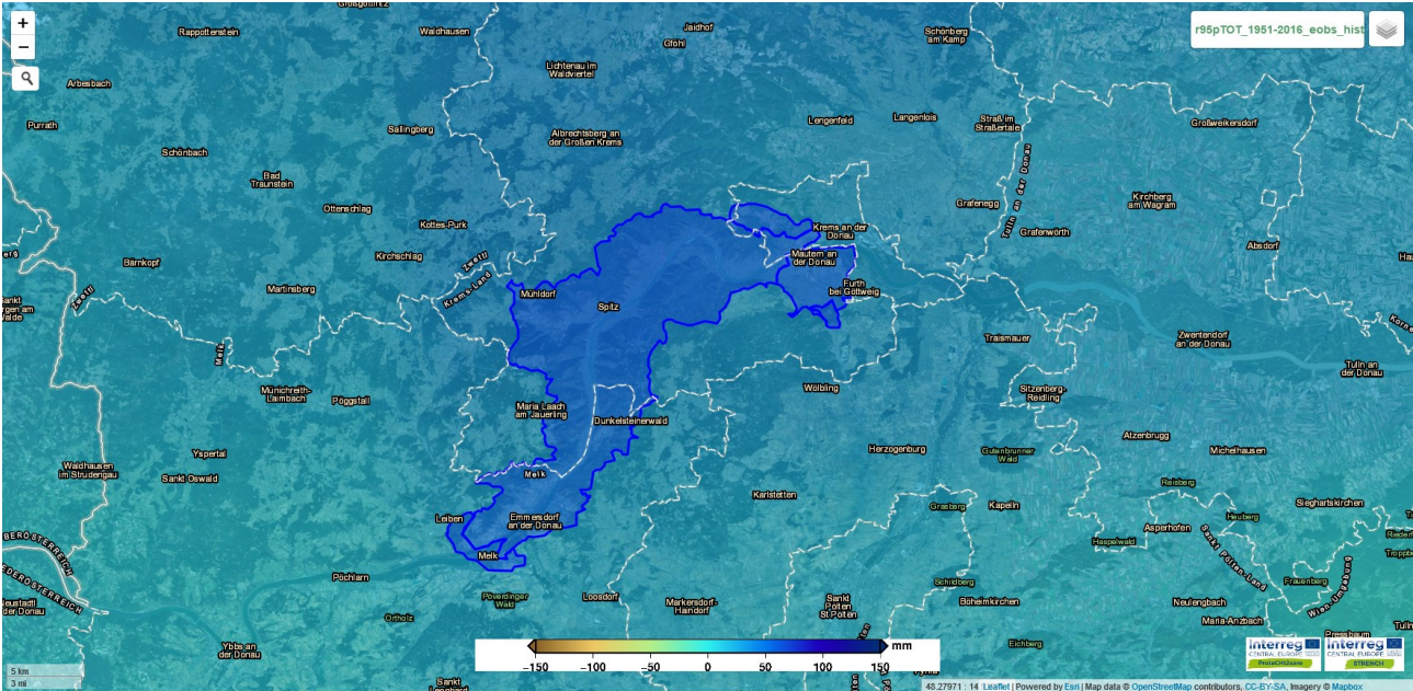
Figure 23 Historical Observation 1951 – 2016, WebGIS tool. (R95pTOT)
