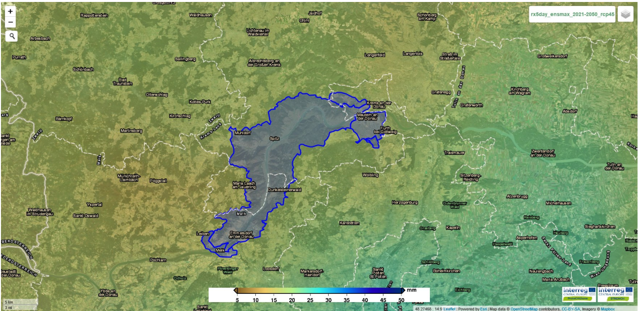
Figure 27 Ensemble statistics, maximum, RCP 4.5 Near Future (2021 – 2050), WebGIS tool. (Rx5day)
