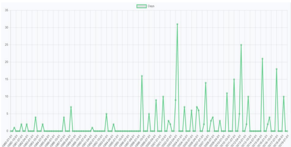
Number of extremely hot days in the year (TXPP90 – ERA5) in the period of 1980-2019
