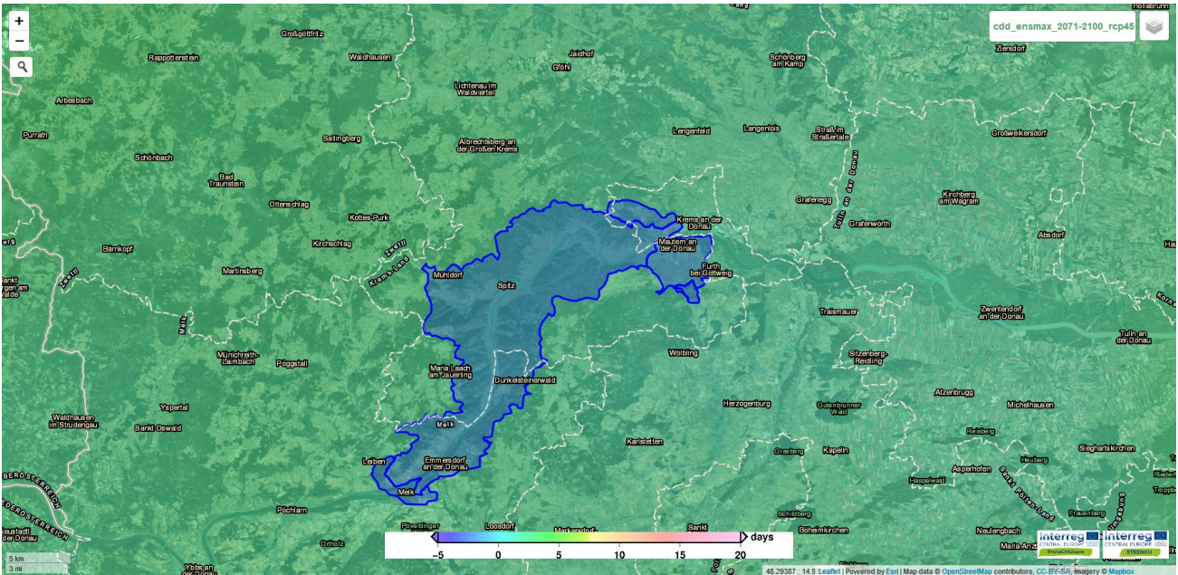
Figure 31 Ensemble statistics, maximum, RCP 4.5 Far Future (2071 – 2100), WebGIS tool (CCD)
