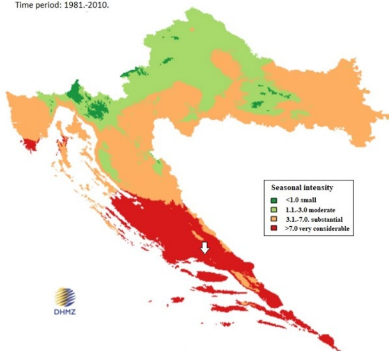
Map of potential fire hazard index Time period: 1981.-2010.
