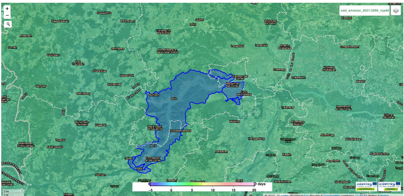
Figure 30 Ensemble statistics, maximum, RCP 4.5 Near Future (2021 – 2050), WebGIS tool. (CCD)
