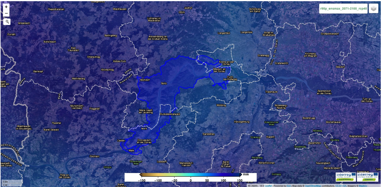
Figure 25 Ensemble statistics, maximum, RCP 4.5 Far Future (2071 – 2100), WebGIS tool. (R95pTOT)
